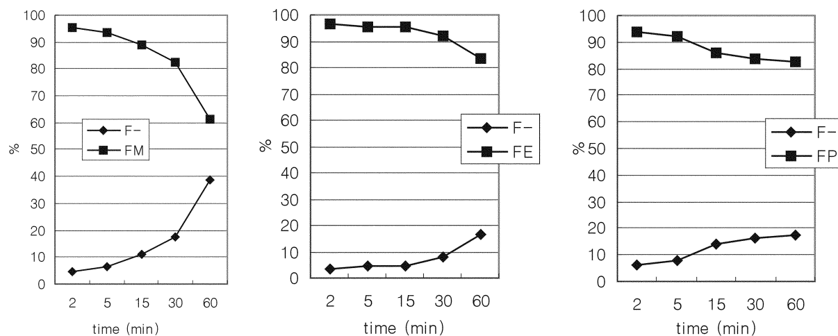
Figure 1. Metabolite analysis of [ 18 F]fluoroalkylbiphenyls (FM = [ 18 F]3a, FE = [ 18 F]3b, FP = [ 18 F]3c).
