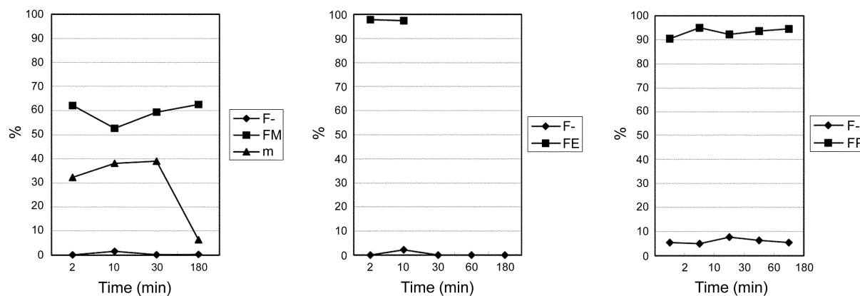
Figure 2. In vitro stability in human serum at 37 °C (FM = [ 18 F]3a, FE = [ 18 F]3b, FP = [ 18 F]3c). The notation m in graph of FM is a metabolite of unknown structure.
