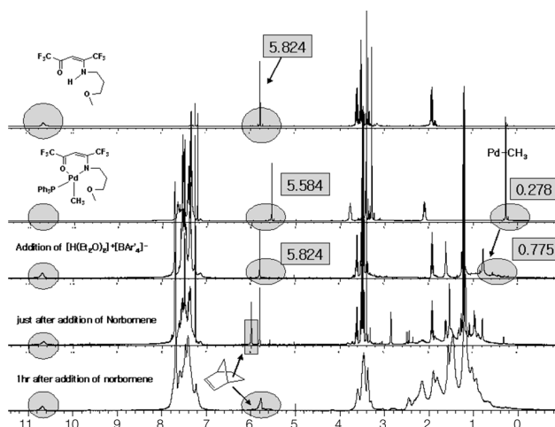
Figure 2. 1 H NMR spectra of the reactions between 13b and [H(Et 2 O) 2 ] + BAR' 4 -
