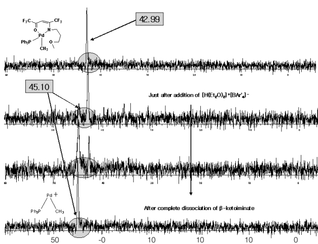
Figure 3. 31 P NMR spectra of the reactions between 13b and [H(Et 2 O) 2 ] + BAR' 4 -
