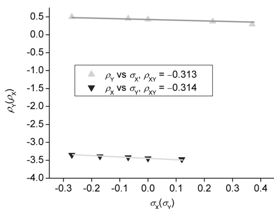
Figure 1. The \rho_{XY} ( = \partial\rho_X/\partial\sigma_Y = \partial\rho_Y/\partial\sigma_X ) plot of \rho_X vs \sigma_Y and \rho_Y vs \sigma_X of the reactions of Y-S-aryl phenyl phosphonochloridothioates ( 1 ) with X-anilines in acetonitrile at 55.0 °C.
