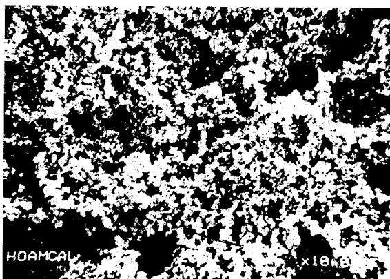
Figure 1. A micrograph of the precipitate obtained in distilled water solution with aging time of 15-60 min at temperature of 25 °C and [\text{DMO}]_0/([\text{Ba}^{2+}]_0 + [\text{Ti}^{4+}]_0) of 4.
