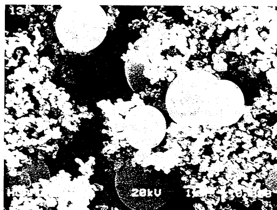
Figure 2. A micrograph of the precipitate obtained in distilled water solution with aging time of 75 min at temperature of 25 °C and [\text{DMO}]_0/([\text{Ba}^{2+}]_0 + [\text{Ti}^{4+}]_0) of 4.
