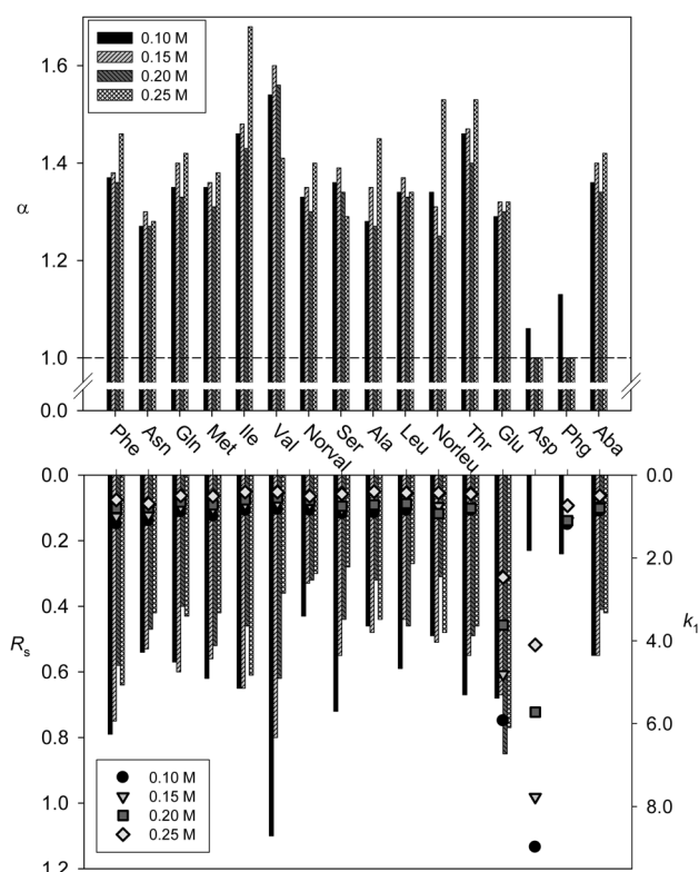
Figure 4. Enantioselectivity ( \alpha ) and resolution ( R_s ) and retention factors ( k_1 ) for the first eluting enantiomers in 80/20 (v/v %) methanol/ammonium acetate buffer (pH 5.0) with varying buffer concentration.
