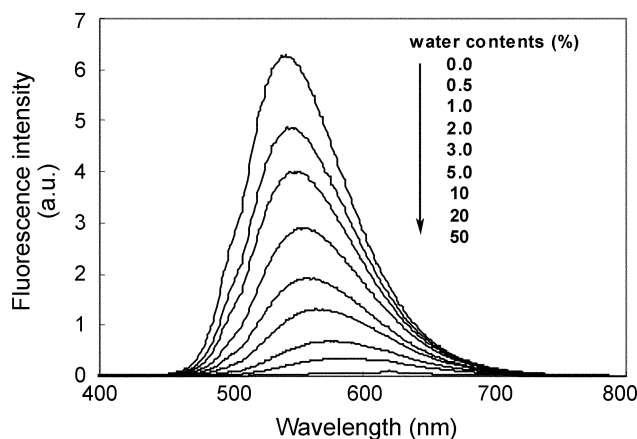
Figure 3. Fluorescence spectra of 3 as a function of water composition in aqueous 1,4-dioxane. [\mathbf{3}] = 2.0 \times 10^{-5} M. \lambda_{ex} = 310 nm.
