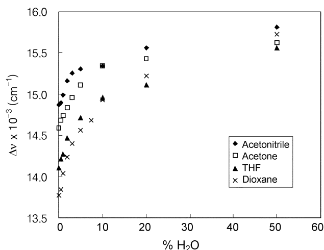
Figure 4. Effects of water composition in aprotic organic solvents on the fluorescence maximum of 3 . [3] = 2.0 \times 10^{-5} M. \lambda_{\text{ex}} = 310 nm.
