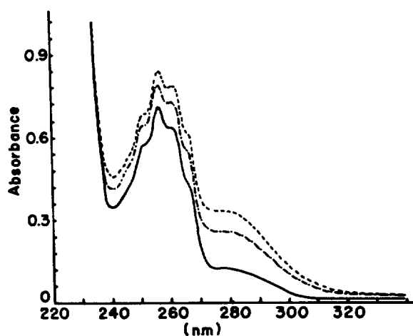
Figure 2. Spectra of N-Cbz-His at \beta -CD concentrations of 1.59 \times 10^{-2} (---), 8.51 \times 10^{-3} (---), and 0 (—) M (concentration of N-Cbz-His: 3.13 \times 10^{-3} M; Tris buffer, pH 10.0). The secondary band of N-Cbz-His is represented.
