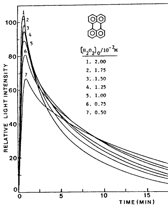
Figure 1. Relative intensity of the peroxyoxalate CL vs. time of 5.0 \times 10^{-5} M perylene, 5.0 \times 10^{-4} M TCPO, 1.2 \times 10^{-4} M sodium salicylate, and various concentrations of H_2O_2 .
