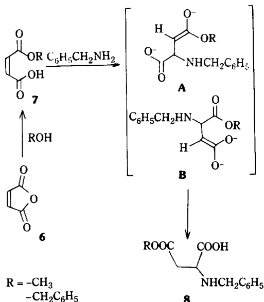
Scheme 1. Synthesis of \beta -Alkyl N-Benzylaspartates
