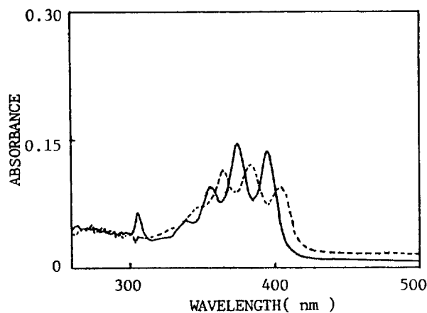
Figure 2. Absorption spectra of 1.0 \times 10^{-5} M of 9,10-diphenylanthracene (solid line) and 9-cyanoanthracene (broken line).
