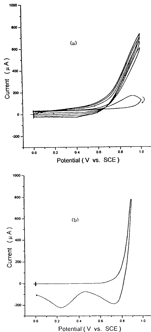
Figure 2. Cyclic voltammograms at gold electrode in aqueous 0.1 M \text{KBr} solutions (pH 7; 30 mM phosphate) in the presence (a) and in the absence (b) of 0.2 M pyrrole. Electrode area: 0.20 \text{cm}^2 , Scan rate: 25 mV/s.
