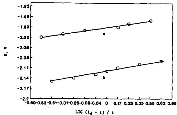
Figure 2. Heyrovsky-Ilkovic plots for the data in Figure 1.
