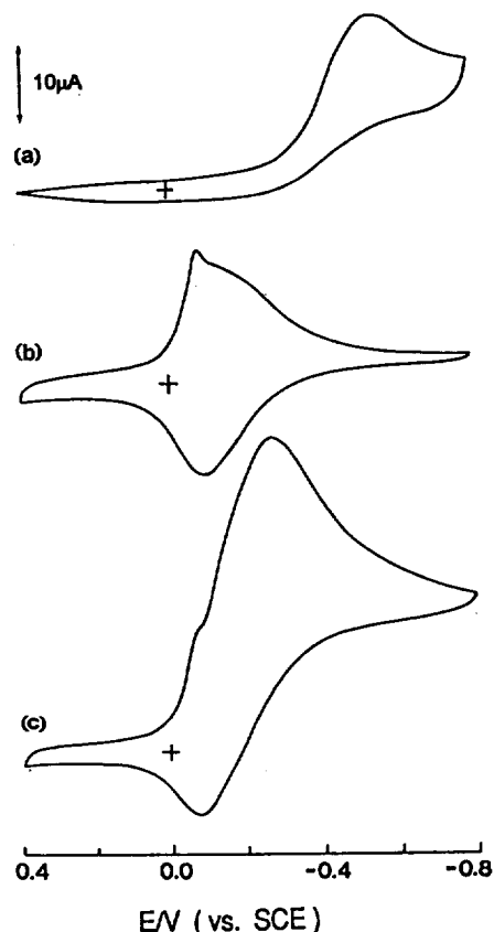
Figure 3. Cyclic voltammograms of the PPD-coated GC electrode in 0.2 M \text{Na}_2\text{SO}_4 solution (pH=1.0). Voltammogram (a) was traced with a bare GC electrode. Potential scan rate; 10 mV/sec. (a) and (c); in \text{O}_2 saturated solution and (b); in \text{N}_2 saturated solution.
