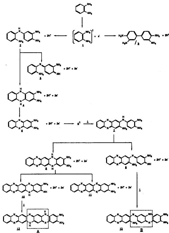
Figure 10. Proposed mechanism for the formation of the active and inactive component during the electropolymerization.
