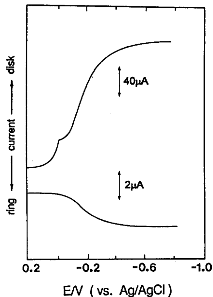
Figure 5. Current-potential curves for the reduction of \text{O}_2 with a rotating PPD-coated GC disk-Pt ring electrode in 0.2 M \text{Na}_2\text{SO}_4 solution (pH=1.0). Rotation speed was 100 rpm.
