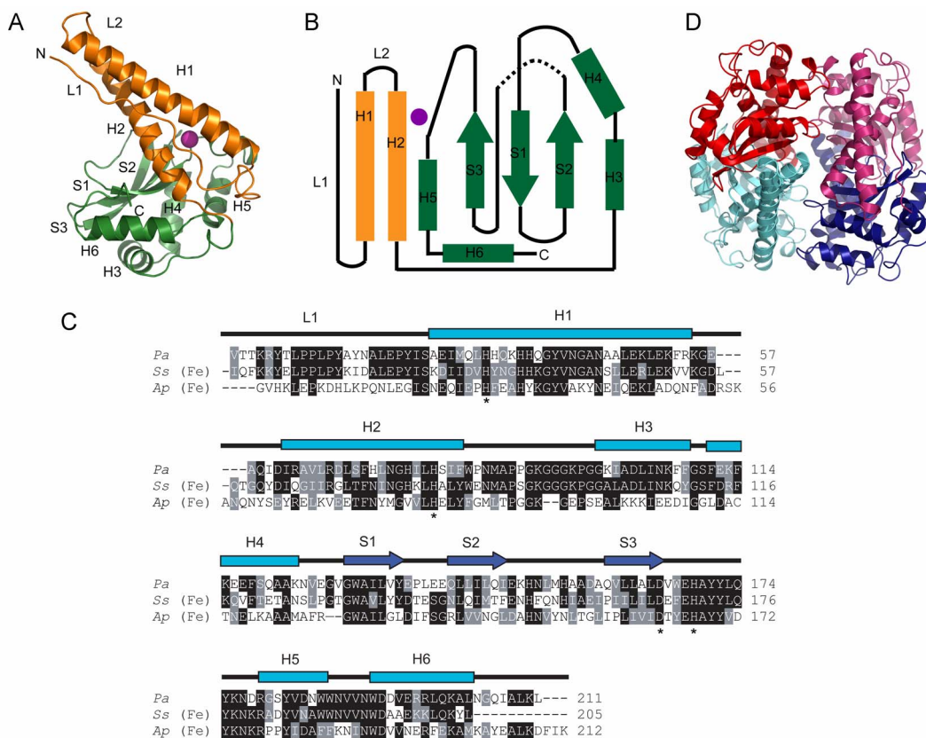
Figure 1. (A) Structure of the metal-bound PaSOD monomer. The N- and C-termini are labeled. N-terminal and C-terminal subdomains are depicted as orange and green, respectively. The manganese is shown as a purple sphere. Secondary structural elements are labeled; H, helix; S, strand; L, loop. (B) Topology of the metal-bound PaSOD monomer. The same coloring scheme as (A) is used to designate the subdomains. (C) Structure-based multiple sequence alignment of Mn-or-Fe SODs. Pa , Pyrobaculum aerophilum ; Ss , Sulfolobus solfataricus ; Ap , Aquifex pyrophilus . Secondary structures of PaSOD are indicated above the alignment with active site residues depicted as asterisks (*). (D) The metal-bound PaSOD tetramer. Chains A and C are colored in blue and cyan, respectively. Chains B and D are presented in red and pink, respectively. Manganese atoms are shown as spheres with the same color as the chain each manganese atom belongs to. This figure was prepared by PyMol ( http://www.pymol.org ).
