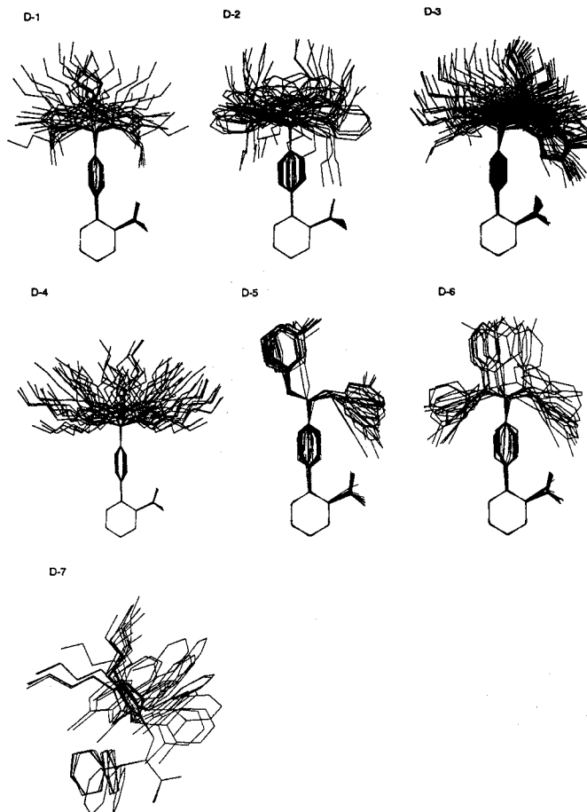
Figure 6. Overlay plot of all thermodynamically possible conformation of nonpeptidic model compounds (see text).
