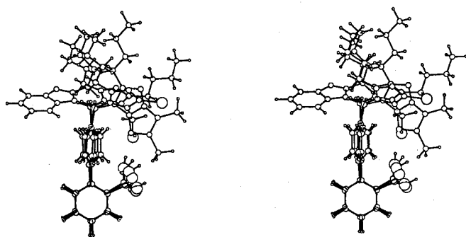
Figure 5. Overlay of model compounds D-1, D-2, D-3, and D-4. Conformations for each compounds are selected from the contour maps in Figure 4. (see also Table 3)
