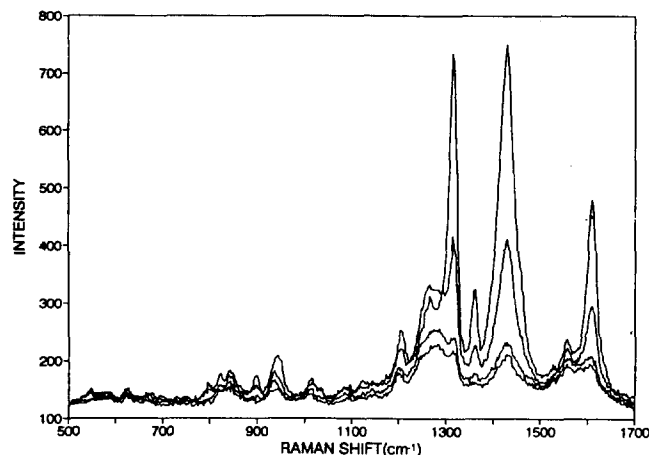
Figure 2. The 3, 50, 100 and 150th SERS spectra (from top to bottom) of o -diiodobenzene adsorbed on silver colloid observed by using the flow system of Figure 1. The exciting laser was operated 488-nm at an input power of 50 mW.
