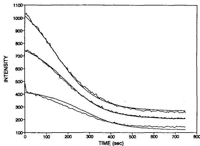
Figure 3. Time evolution of the SERS intensity at 1427 \text{ cm}^{-1} excited with 488-nm \text{Ar}^+ laser line. Jagged lines are experimental data; smooth lines are recalculated according to the model described in the text. The laser power from top to bottom: 75, 50, 25 mW.
