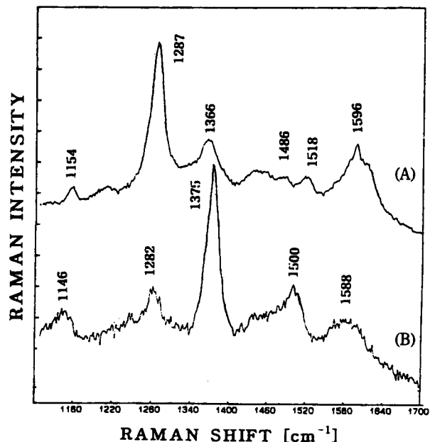
Figure 1. Raman spectra of dopamine adsorbed on Ag adatoms (A) and on Cu adatoms (B) deposited on the silver electrode at -0.9 V vs SCE. ( \lambda_{\text{ex}}=514.5 nm, 1 mM dopamine concentration in pH 7.2 phosphate buffer).
