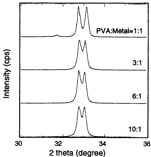
Figure 10. PXRD patterns of \text{La}_{0.8}\text{Sr}_{0.2}\text{CoO}_3 , prepared by annealing the samples used for taking the PXRD patterns in the Figure 9, at 1000\text{ }^\circ\text{C} for 1h in air. Only (110) and (104) diffractions were obtained with slow scan rate.
