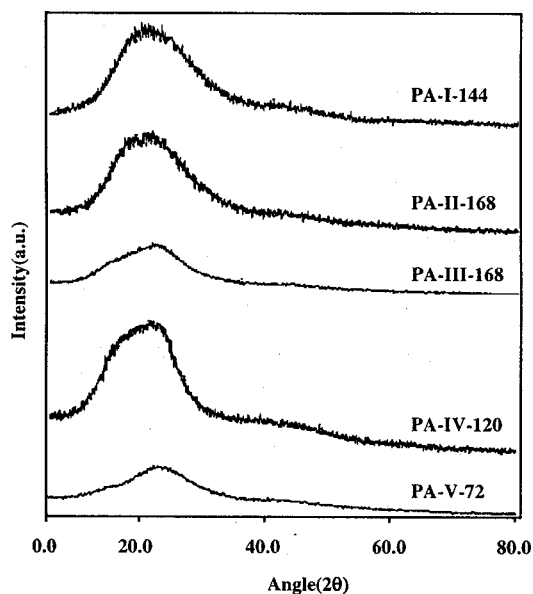
Figure 5. Wide angle X-ray diffractograms of poly(4-nitrophenylallylamine) derivatives.
