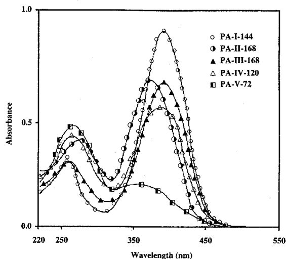
Figure 3. UV/vis. absorption spectra of poly(4-nitrophenylallylamine) derivatives.
