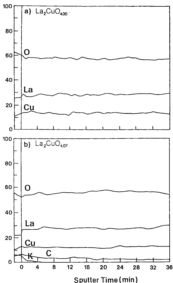
Figure 11. Atomic percentage of \text{La}_2\text{CuO}_{4+\delta} before and after electrochemical oxidation.
