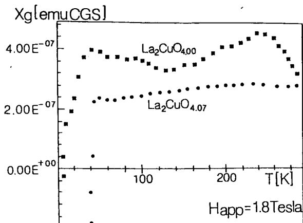
Figure 12. Thermal evolution of magnetic susceptibility of \text{La}_2\text{CuO}_{4+\delta} at T > T_c .
