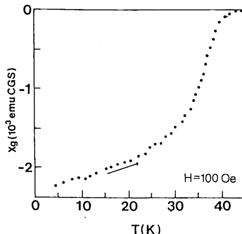
Figure 4. Temperature dependence of the diamagnetic susceptibility of \text{La}_2\text{CuO}_{4.8} after electrochemical oxidation.
