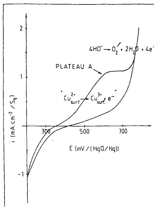
Figure 1. Cyclic voltammogram for \text{La}_2\text{CuO}_4 in 1 N KOH ( 6 \text{ mVs}^{-1} ).
