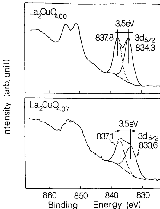
Figure 6. La(3d) XPS spectra of \text{La}_2\text{CuO}_{4+\delta} before and after electrochemical oxidation.
