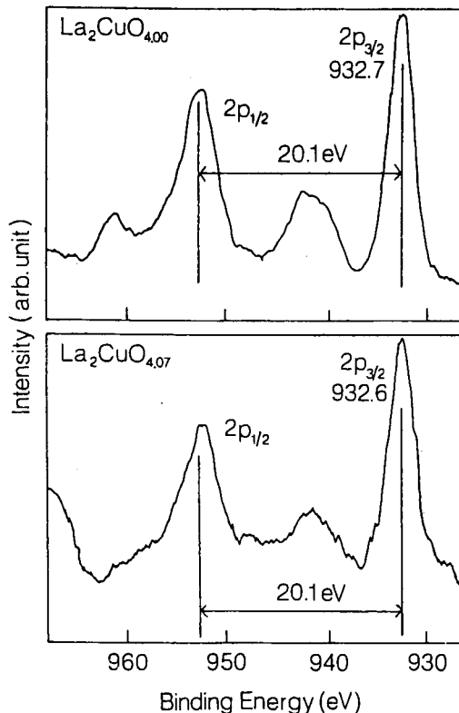
Figure 7. Cu(2p) XPS spectra of \text{La}_2\text{CuO}_{4+\delta} before and after electrochemical oxidation.
