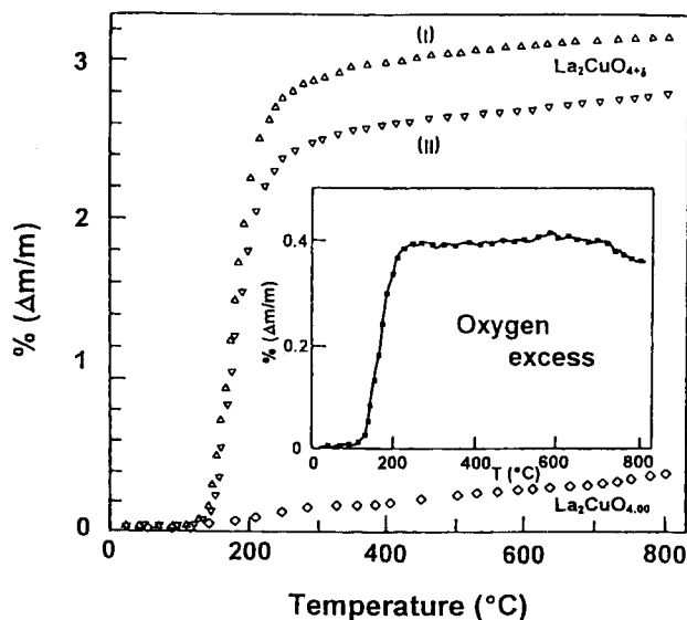
Figure 5. The excess oxygen content in \text{La}_2\text{CuO}_{4.8} .
