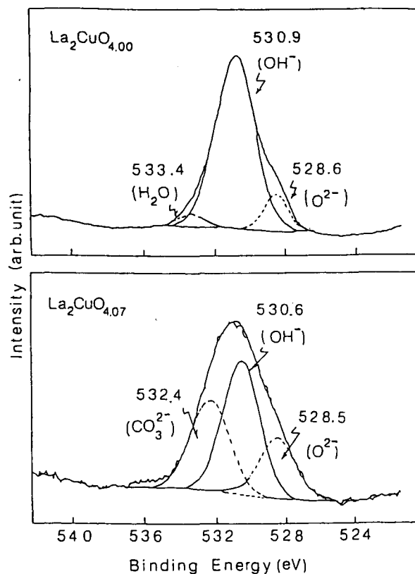
Figure 9. O(1s) XPS spectra of \text{La}_2\text{CuO}_{4+\delta} before and after electrochemical oxidation.
