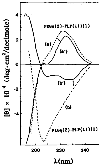
Figure 2. CD spectra of the PLP(II)/PLGA (PDGA) 1 : 2 binary complex systems in water-methanol (1 : 2 v/v) at 25 °C. Dotted lines denote the ideal spectra obtained using Eq. (1), and solid lines denote the actual spectra. The number in the parentheses appearing in the figure represent the unit mole fractions of the corresponding polypeptides in a given binary complex system.
