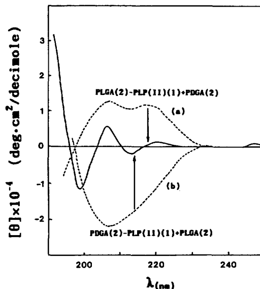
Figure 3. CD spectra for the ternary complex system of PDGA, PLGA, and PLP(II) in water-methanol (1 : 2 v/v) at 25 °C. Dotted lines represent the ideal spectra obtained from the simple adding-up of the spectra for (a) PLGA-PLP(II) and PDGA and (b) PDGA-PLP(II) and PLGA with respect to unit mole fractions (as given by the numbers in the parentheses).
