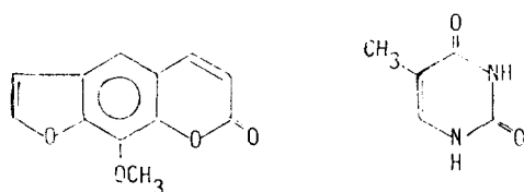
8-MOP
