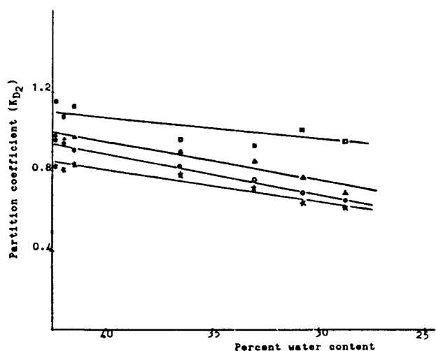
Figure 1. The partition coefficient of solute as a function of equilibrium water content of membranes at 25 °C; (□) 1,3-dimethylurea; (Δ) methylurea; (o) urea; (*) acetamide.
