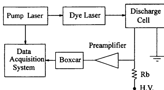
Figure 1. Schematic diagram of the experimental layout for the pulsed optogalvanic spectroscopy. R_b is 5\text{ k}\Omega and H. V. is about 400 volts.
