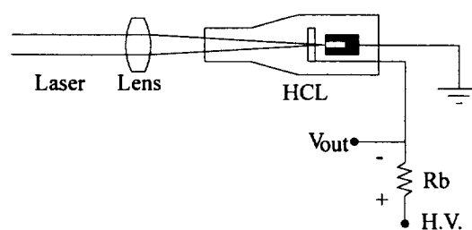
Figure 2. Optical alignment of the experimental apparatus.
