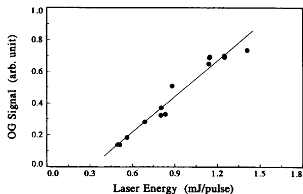
Figure 5. Effect of the pulse energy on the OG signal with titanium. The discharge current was 5 mA.
