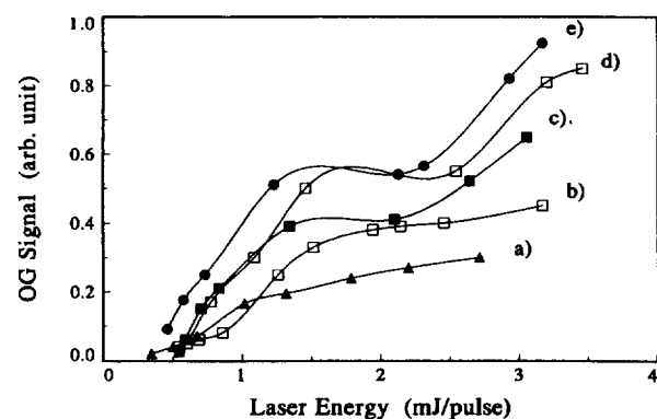
Figure 6. OG signal of Ti vs. pulse energy at different discharge current. (a) 3.8 mA, (b) 6.8 mA, (c) 12.4 mA, (d) 17.2 mA, and (e) 20.1 mA.
