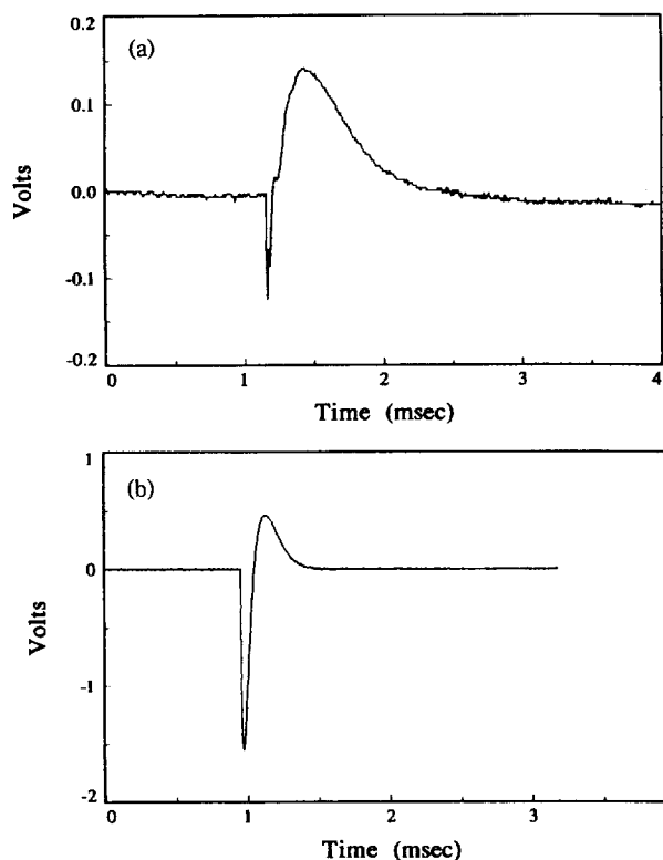
Figure 3. Shape of OG signals from different elements. (a) Ti; 564.414 nm and (b) Ba; 577.700 nm. The discharge current was 5 mA for (a) and 10 mA for (b).
