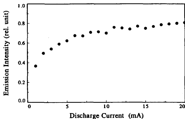
Figure 7. Current dependence of emission intensity of Fe hollow cathode lamp ( \lambda=372.0 nm).
