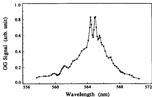
Figure 4. OG spectrum of Ti around 564 nm. The discharge current was 5 mA.
