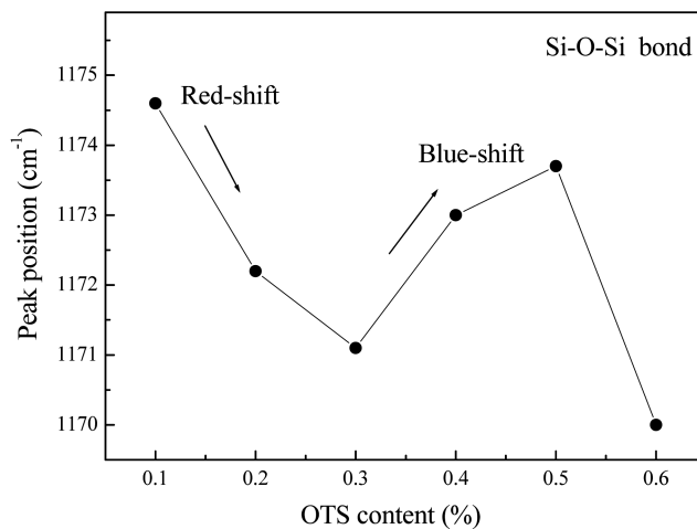
Figure 3. Chemical shift by the peak position of Si-O-Si bond.
