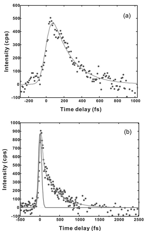
Figure 4. S_2 -fluorescence decay profiles of \text{Sn(TPP)(FcCOO)}_2 (a) and \text{Sn(TPP)Cl}_2 (b) measured by up-conversion technique. \lambda_{\text{ex}} = 410 nm.
