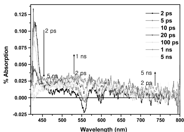
Figure 6. fs-Transient absorption spectra of \text{Sn(TPP)(FcCOO)}_2 upon excitation at 390 nm.
