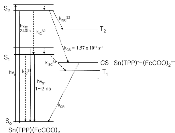
Figure 7. Schematic energy diagram for the deactivation processes in competition with the S_1 - and S_2 -fluorescence ( h\nu_{S_1} , h\nu_{S_2} ) of \text{Sn(TPP)(FcCOO)}_2 including CS formation and charge recombination (CR) with internal conversion (IC) and intersystem crossing (ISC).
