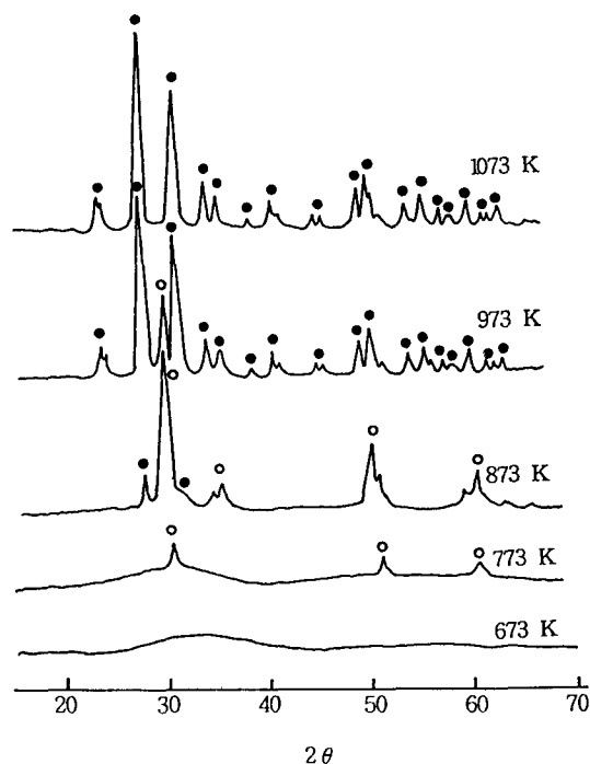
Figure 3. X-ray diffraction patterns of 9- V_2O_5 - ZrO_2 calcined at different temperature for 1.5 hr. ○ : tetragonal phase ZrO_2 , ● : monoclinic phase ZrO_2 .
