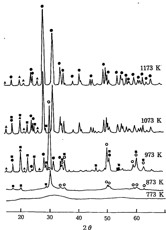
Figure 4. X-ray diffraction patterns of 15- V_2O_5 - ZrO_2 calcined at different temperature for 1.5 hr. ○ : tetragonal phase ZrO_2 , ● : monoclinic phase ZrO_2 , △ : orthorhombic phase V_2O_5 , ■ : cubic phase ZrV_2O_7 .
