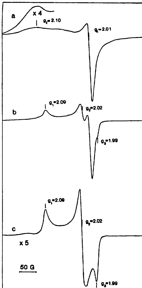
Figure 6. ESR spectra obtained at 123 K after controlled potential reduction of (a) O_2 in THF at -0.65 V, (b) Rh_2(ap)_4 in THF under O_2 at -0.65 V and (c) Rh_2(ap)_4(O_2) in THF under O_2 at -0.25 V after bulk electrolysis at -0.65 V.
