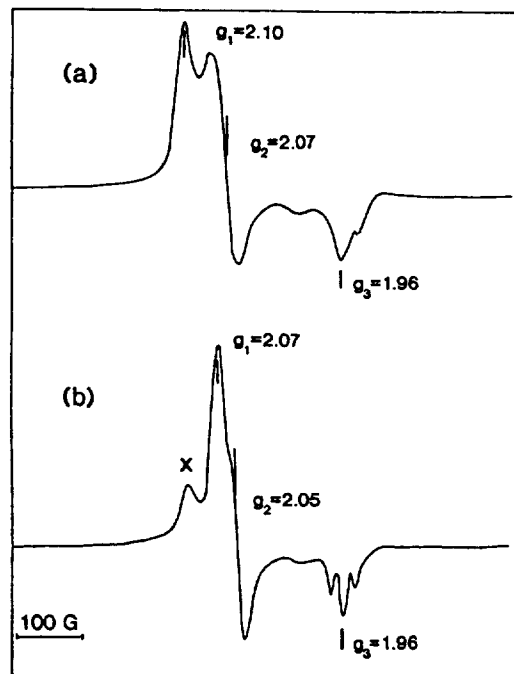
Figure 7. ESR spectra obtained at 123 K after controlled potential oxidation of Rh_2(ap)_4 (a) in CH_2Cl_2 and (b) in CH_2Cl_2 containing 5 \times 10^{-3} M CH_3CN . Applied potential = 0.55 V under O_2 .
