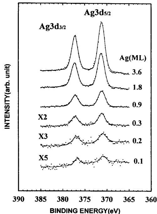
Figure 2. X-ray photoelectron spectra of Ag 3d core levels for Ag adlayers deposited on Pt(211) with \theta=0.1, 0.2, 0.3, 0.9, 1.8, and 3.6 ML.
