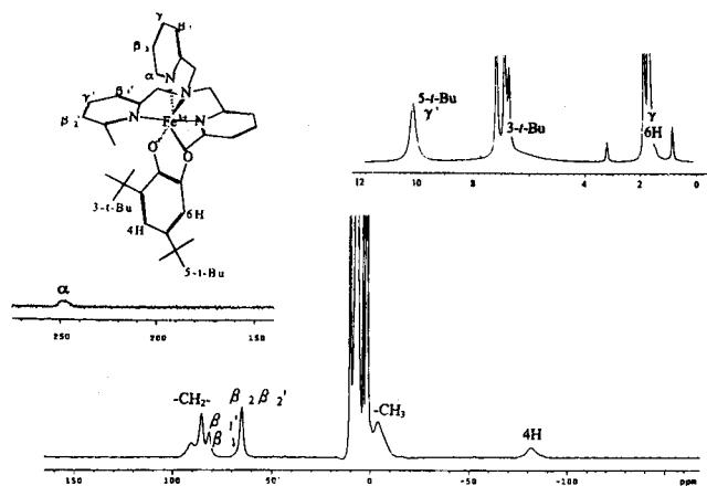
Figure 2. ^1\text{H} NMR spectrum of [\text{Fe}(\text{BLPA})\text{DBC}]\text{BPh}_4 in \text{CD}_3\text{CN} under argon with ambient conditions. The right inset is an expansion of diamagnetic region of the main spectrum. The two peaks at 7.3 and 6.9 ppm correspond to the protons of \text{BPh}_4 counter anion.
