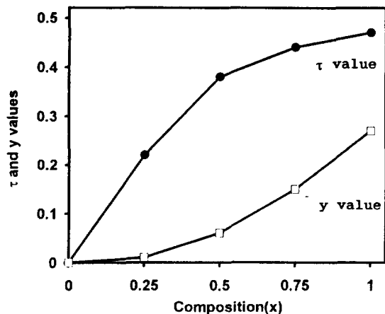
Figure 1. Plot of the \tau and y values vs. x value for the \text{Nd}_{1-x}\text{Sr}_x\text{Fe}^{3+}_{1-\tau}\text{Fe}^{4+}_\tau\text{O}_{3-y} system.
