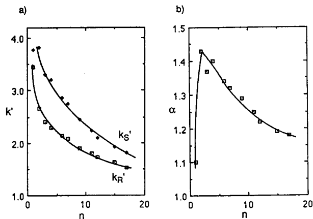
Figure 1. Trends in (a) the capacity factors of the two enantiomers and in (b) the separation factors for resolving N-acyl- \alpha -(1-naphthyl)ethylamines 6 ( R=CH_3 ) on CSP 1. The length of the acyl chain [ Y: -(CH_2)_nH ] of the analyte is denoted by n on the abscissa. For the chromatographic conditions, see Experimental and the footnote to Table 1.
