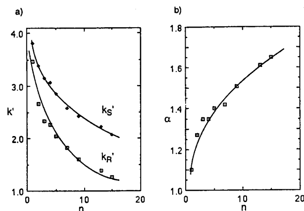
Figure 2. Trends in (a) the capacity factors of the two enantiomers and in (b) the separation factors for resolving N-acetyl- \alpha -(1-naphthyl)alkylamines 6 ( Y=CH_3 ) on CSP 1. The length of the alkyl chain [ R: -(CH_2)_nH ] at the chiral center of the analyte is denoted by n on the abscissa. For the chromatographic conditions, see Experimental and the footnote to Table 1.
