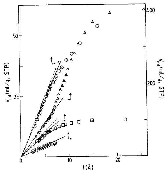
Figure 5. The V-t plot based on de Boer's universal adsorption isotherm. \diamond , BN; \square , \gamma -alumina; \triangle , Silicagel(A); \circ , Silicagel(B).
