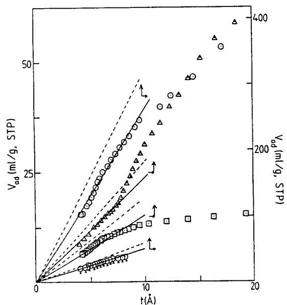
Figure 3. The V-t plot based on Shull's universal adsorption isotherm. \diamond , BN; \square , \gamma -alumina; \triangle , Silicagel(A); \circ , Silicagel(B).
