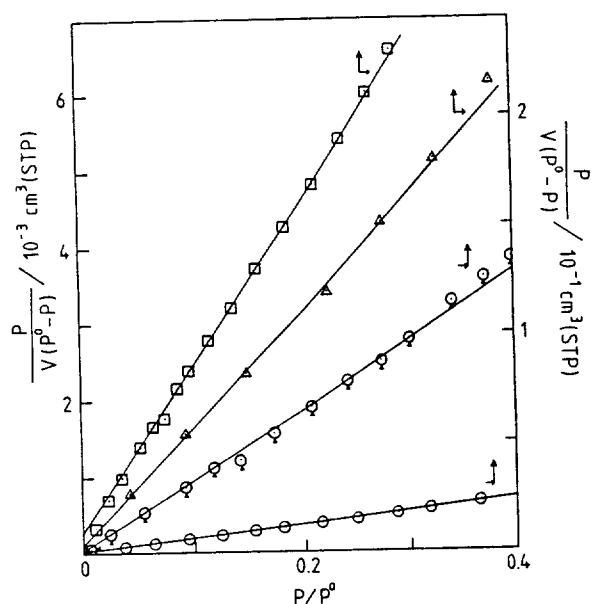
Figure 2. BET plot. \diamond , BN; \square , \gamma -alumina; \triangle , Silicagel(A); \circ , Silicagel(B).
