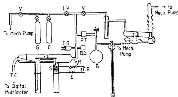
Figure 1. Schematic diagram of the adsorption apparatus. M.B.: quartz beam microbalance, V.R.: variable resistance, F.R.: fixed resistance, V: Hoke valve, L.V.: leak valve, I.G.: ionization gauge, B.G.: Baratron gauge, P.T.: pressure transducer, M: magnet, S: solenoid, E: battery, B: ballast, G: gas, T.C.: thermocouple
