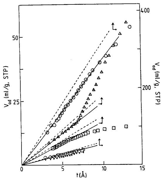
Figure 4. The V-t plot based on Cranston & Inkley's universal adsorption isotherm. \diamond , BN; \square , \gamma -alumina; \triangle , Silicagel(A); \circ , Silicagel(B).
