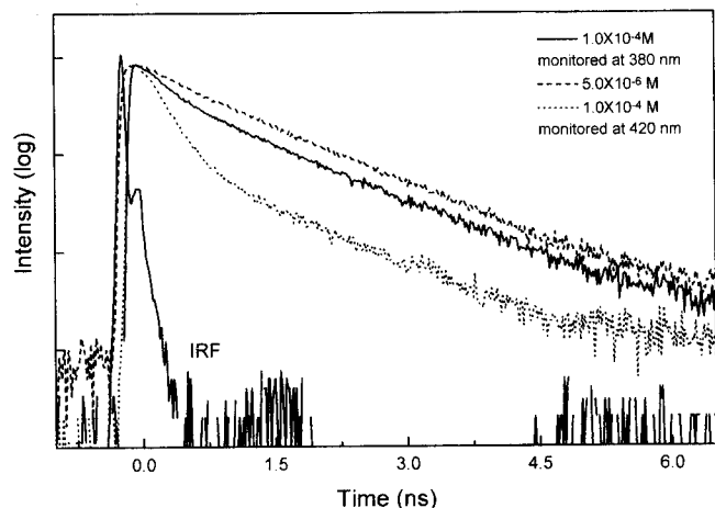
Figure 7. The fluorescence decay curve of aminosalicyclic acid monitored at 380 nm and 420 nm. The excitation wavelength is 300 nm.
