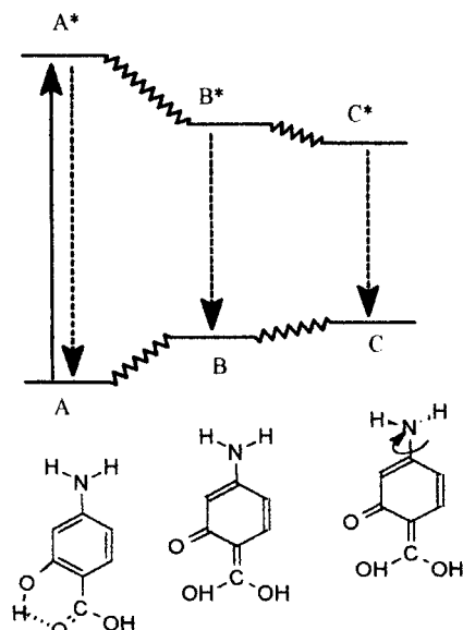
Scheme 2. Potential energy diagram of proton-transfer coupled ICT of AS.
