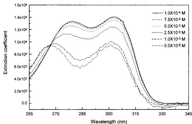
Figure 3. Absorption spectra of aminosalicic acid in methanol as a function of concentration.
