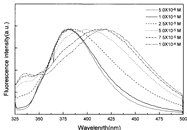
Figure 4. Fluorescence emission spectra of aminosalicic acid in ethanol as a function of concentration. The excitation wavelength is 300 nm.
