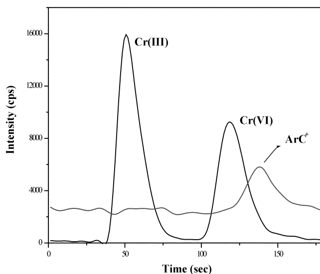
Figure 5. A chromatogram for 10 \mu\text{g/L} Cr(III) and Cr(VI) in 0.001 M \text{HNO}_3 including carbonate ion ( \text{CO}_3^{2-} ) with ICP-MS and IC. (Concentration of carbon: 15 mg/L). Eluent: 0.06 M \text{HNO}_3 , Resolution: 4000.
