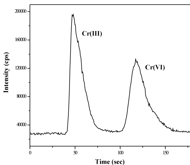
Figure 2. A chromatogram for 10 \mu\text{g/L} Cr(III) and Cr(VI) in 0.001 M \text{HNO}_3 including carbonate ion ( \text{CO}_3^{2-} ) with ICP-MS and IC. (Concentration of carbon: 5 mg/L. Eluent: 0.06 M \text{HNO}_3 , Resolution: 300.
