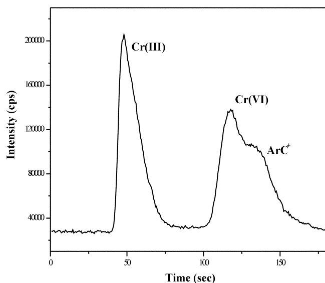
Figure 3. A chromatogram for 10 \mu\text{g/L} Cr(III) and Cr(VI) in 0.001 M \text{HNO}_3 including carbonate ion ( \text{CO}_3^{2-} ) with ICP-MS and IC. (Concentration of carbon: 15 mg/L). Eluent: 0.06 M \text{HNO}_3 , Resolution: 300.
