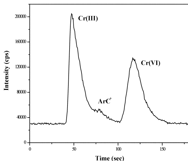
Figure 4. A chromatogram for 10 \mu\text{g/L} Cr(III) and Cr(VI) in 0.001 M \text{HNO}_3 including carbonate ion ( \text{CN}^- ) with ICP-MS and IC. (Concentration of carbon: 5 mg/L). Eluent: 0.06 M \text{HNO}_3 , Resolution: 300.
