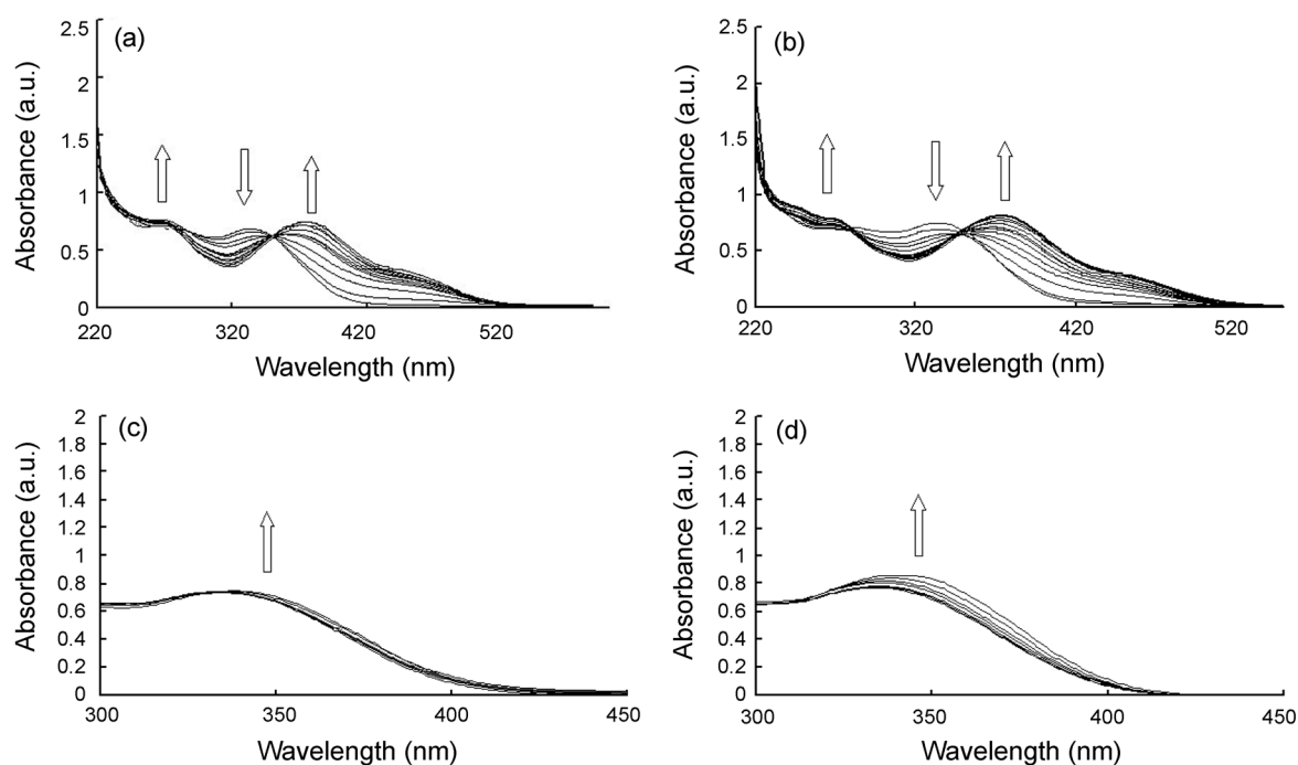
Figure 1. Family of spectra taken in the course of the titration of a \text{CH}_3\text{CN} solution 1.0 \times 10^{-4} in receptor 1 , \mathbf{1} + \text{Na}^+ with a standard solution of acetate: (a) acetate titration only. (from 0 eq to 5 eq) (b) acetate titration in the presence of \text{Na}^+ . (from 0 eq to 5 eq) (c) iodide titration only. (from 0 eq to 100 eq) (d) iodide titration in the presence of \text{Na}^+ . (from 0 eq to 100 eq)
