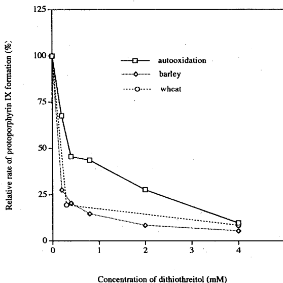
Figure 1. Effect of DTT on the rate of Protogen oxidation. The rates of Protogen oxidation were measured at various concentrations of DTT and calculated by leastsquare method using data-points for the initial 5 minutes. Reaction mixture contained 100 mM HEPES (pH 7.5), 5 mM EDTA, 1% Tween-20, and 120 \mu L of etioplast extract (0.62 mg of protein) in 3 mL. The reaction was started by adding 300 \mu L of 200 \mu M substrate. Fluorescence intensity was monitored using spectrofluorometer at 626 nm with excitation at 395 nm. Rates of autooxidation ( \square ) and enzymatic oxidation (barley ( \diamond ), wheat ( \circ )) were expressed relative to those at zero concentration of DTT.
