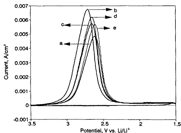
Figure 4. Cyclic voltammograms for the reduction of \text{SOCl}_2 solution at optimum concentration containing: a) bare, b) [\text{Co}(\text{II})(\text{SOPD})] , c) [\text{Co}(\text{II})_2(\text{SPPD})_2] , d) [\text{Ni}(\text{II})(\text{SOPD})] , and e) [\text{Ni}(\text{II})_2(\text{SPPD})_2] . Scan rate was 50\text{ mV/s} .
