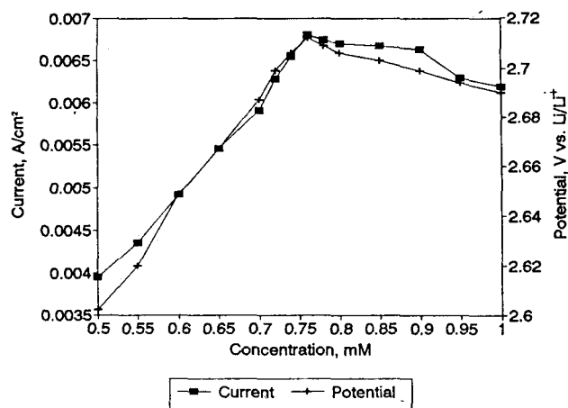
Figure 3. Plots of the peak currents and peak potentials vs. the concentration of catalysts for the reduction of \text{SOCl}_2 solution containing [\text{Co}(\text{II})(\text{SOPD})] at glassy carbon electrode. Scan rate was 50\text{ mV/sec} .
