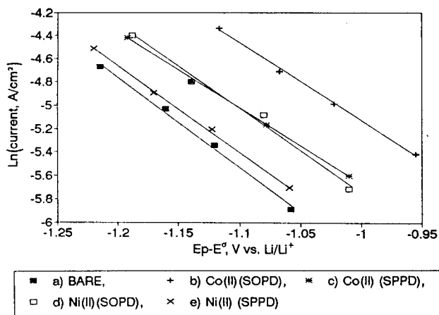
Figure 7. Plots of \ln(i_p) vs. (E_p - E^\circ) for the reduction of \text{SOCl}_2 at optimum concentration containing: a) bare, b) [\text{Co(II)(SOPD)}] , c) [\text{Co(II)}_2(\text{SPPD})_2] , d) [\text{Ni(II)(SOPD)}] , and e) [\text{Ni(II)}_2(\text{SPPD})_2] .
