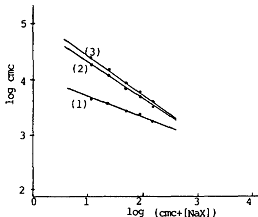
Figure 2. log cmc (of CPB) as a function of log (total counterion conc. at the cmc) for added NaCl (1), NaBr (2), and NaNO 3 (3) at 25°C.
