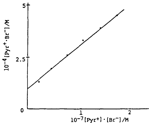
Figure 3. Plot of [P yr + ·Br - ] vs [P yr + ][Br - ] in water at 25°C.
