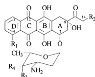
1a: Adriamycin R_1 = \text{OMe}, R_2 = R_3 = \text{OH}, R_4 = \text{H} 1b: Daunorubicin R_1 = \text{OMe}, R_2 = R_4 = \text{H}, R_3 = \text{OH} 1c: Carminomycin R_1 = R_3 = \text{OH}, R_2 = R_4 = \text{H} 1d: Epirubicin R_1 = \text{OMe}, R_2 = R_4 = \text{OH}, R_3 = \text{H} 1e: Idarubicin R_1 = R_2 = R_4 = \text{H}, R_3 = \text{OH}
