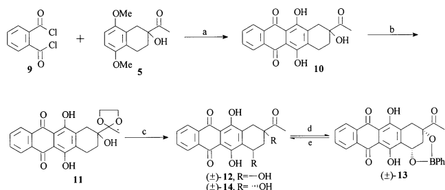
Scheme 2. (a) \text{AlCl}_3 , nitrobenzene, rt. (b) Ethylene glycol, p -TsOH \cdot \text{H}_2\text{O} , benzene. (c) \text{Br}_2 , AIBN, \text{CCl}_4 , silica gel/wet THF, HCl/dioxane. (d) \text{PhB}(\text{OH})_2 , p -TsOH/toluene, rt. (e) 2-Methyl-2,4-pentanediol, \text{AcOH}/\text{CH}_2\text{Cl}_2/\text{acetone} .
