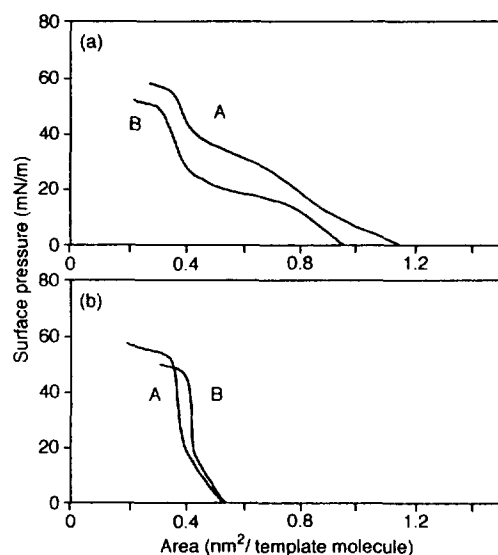
Figure 1. Surface pressure-area isotherms of 2C 18 DAE fixed electrostatically with itaconic acid copolymers: (a) IA-BVE. (b) IA-EVE; A, on pure water; B, on aqueous PAA at 30 °C. The concentration of the amino group of PAA is 2 \times 10^{-4} M.
