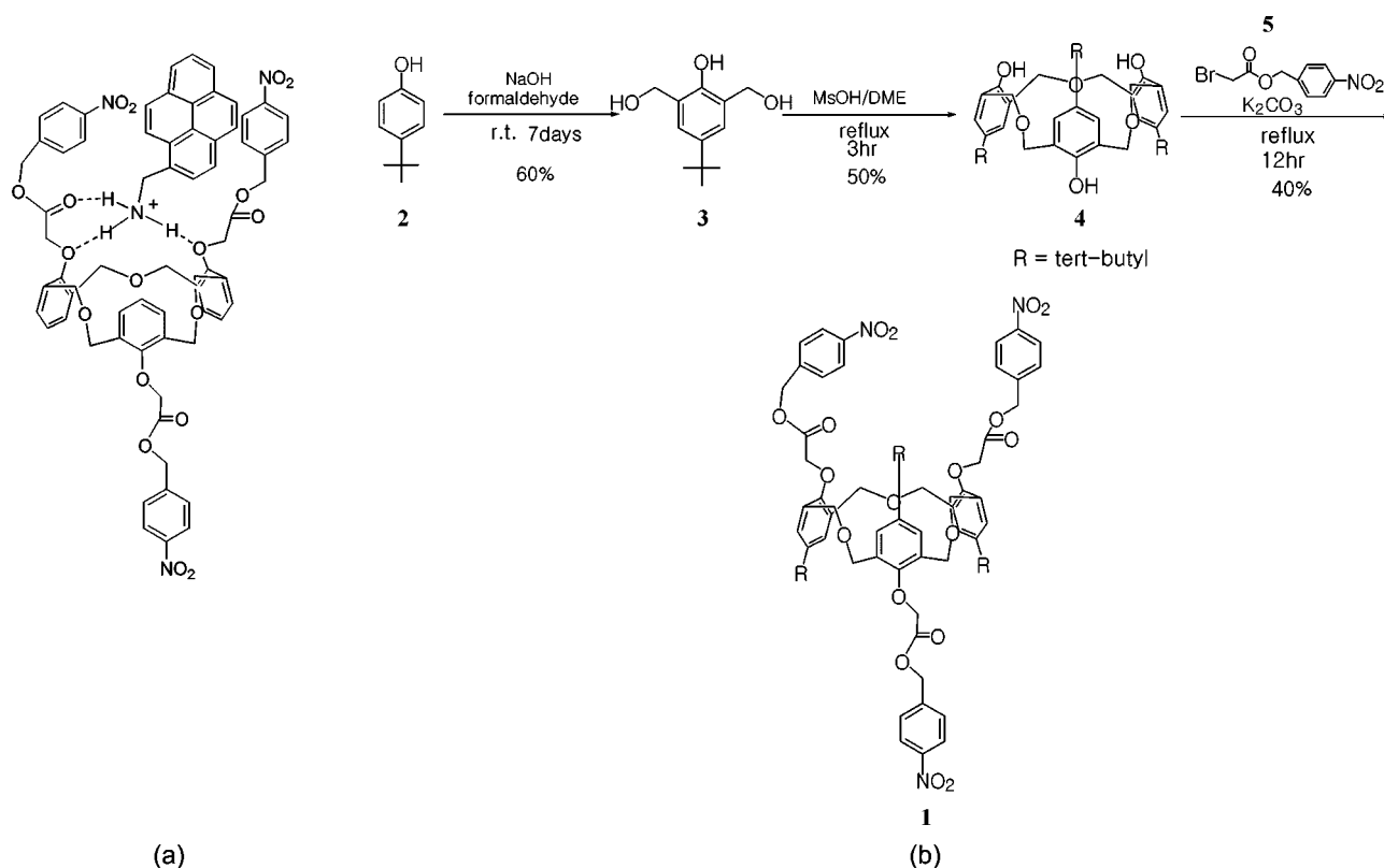
Figure 1. (a) The proposed binding mode of pyrenemethylamine hydrochloride and nitrobenzene modified calixarene 1 . The tert-butyl group was omitted for clarity. (b) The synthetic scheme for the preparation of 1 .
