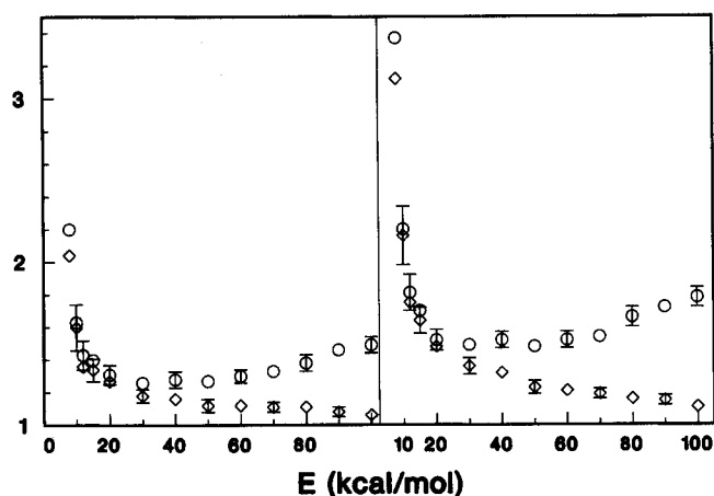
Figure 4. Intermolecular isotope effects, I_T , defined in Eq. 7 and reorientation effects on I_T in the reaction of Y+H_2 ( v=0, J=0 ) \rightarrow YH+H as a function of relative collision energy below 100 kcal/mol. The left panel shows I_T(T)=Q_R(T+H_2)/Q_R(H+H_2) and the right panel shows I_T(X)=Q_R(X+H_2)/Q_R(H+H_2) where X is a fictitious hydrogen isotope atom with 20 amu. Circles and diamonds correspond to I_T and reorientation effect, respectively. The gap between diamond and circles at each collision energy corresponds to the recrossing effect on I_T .
