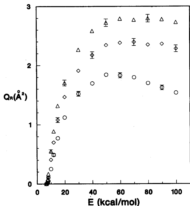
Figure 3. Reaction cross section for Y+H_2 ( v=0, J=0 ) \rightarrow YH+H as a function of relative collision energy below 100 kcal/mol. Circles, diamonds, and triangles correspond to Y=H, T, and X=20 amu, respectively. The 68% confidence limits are shown selectively.
