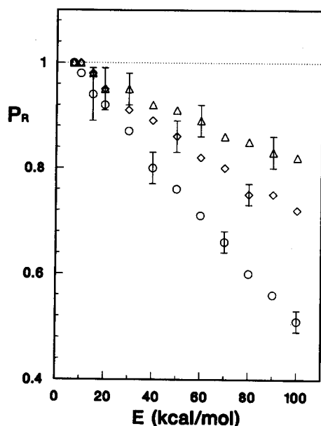
Figure 5. Reaction probability, P_R , defined in Eq. 5 plotted against the relative collision energy below 100 kcal/mol for Y+H_2 ( \nu=0, J=0 ) \rightarrow YH+H . Circles, diamonds, and triangles correspond to Y=H, T, and X=20 amu, respectively. The 68% confidence limits are shown selectively.
