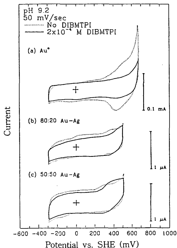
Figure 4. Cyclic voltammograms of (a) \text{Au}^0 , (b) 80 : 20 Au-Ag, and (c) 50 : 50 Au-Ag at pH 9.2 in 0 (---) and 2 \times 10^{-4} M (—) DIBMTPI.
