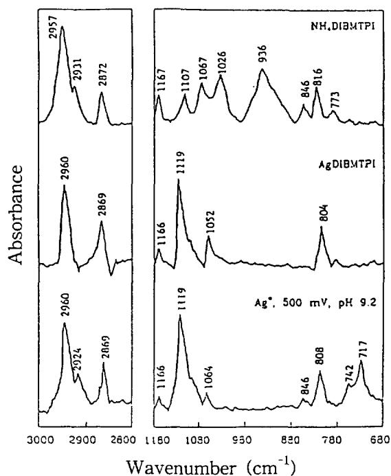
Figure 5. FTIR spectra of \text{NH}_4\text{DIBMTPI} , \text{AgDIBMTPI} , and \text{Ag}^+ conditioned in 2 \times 10^{-4} M DIBMTPI at pH 9.2 and 500 mV.
