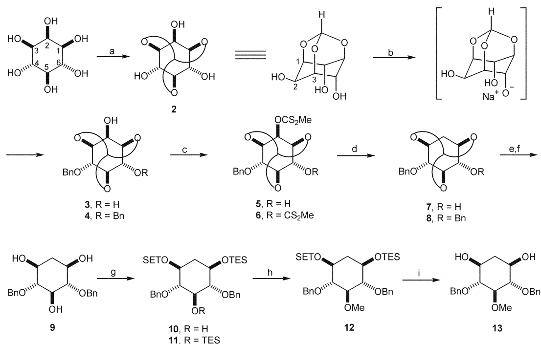
Scheme 1 7 . Reagents and conditions: (a) \text{HC}(\text{OEt})_3 , p -TsOH (cat.), DMF, 80%; (b) NaH (1.1 eq.), BnBr (1.1 eq.), DMF, 25 °C, 85% ( 3 : 4 = 8 : 1); (c) NaH (1.1 eq.), \text{CS}_2 (1.1 eq.), MeI, reflux, 85% ( 5 : 6 = 8 : 1); (d) (n\text{-Bu})_3\text{SnH} , AIBN, toluene, reflux, 90%; (e) NaH (1.2 eq.), BnBr (1.2 eq.), DMF; (f) aq. HCl, two steps 93%; (g) TESCl (2.2 eq.), pyridine, 85% ( 10 : 11 = 7 : 1); (h) NaH (1.2 eq.), MeI (1.2 eq.), DMF, 94%; (i) (n\text{-Bu})_4\text{NF} , THF, 100%.
