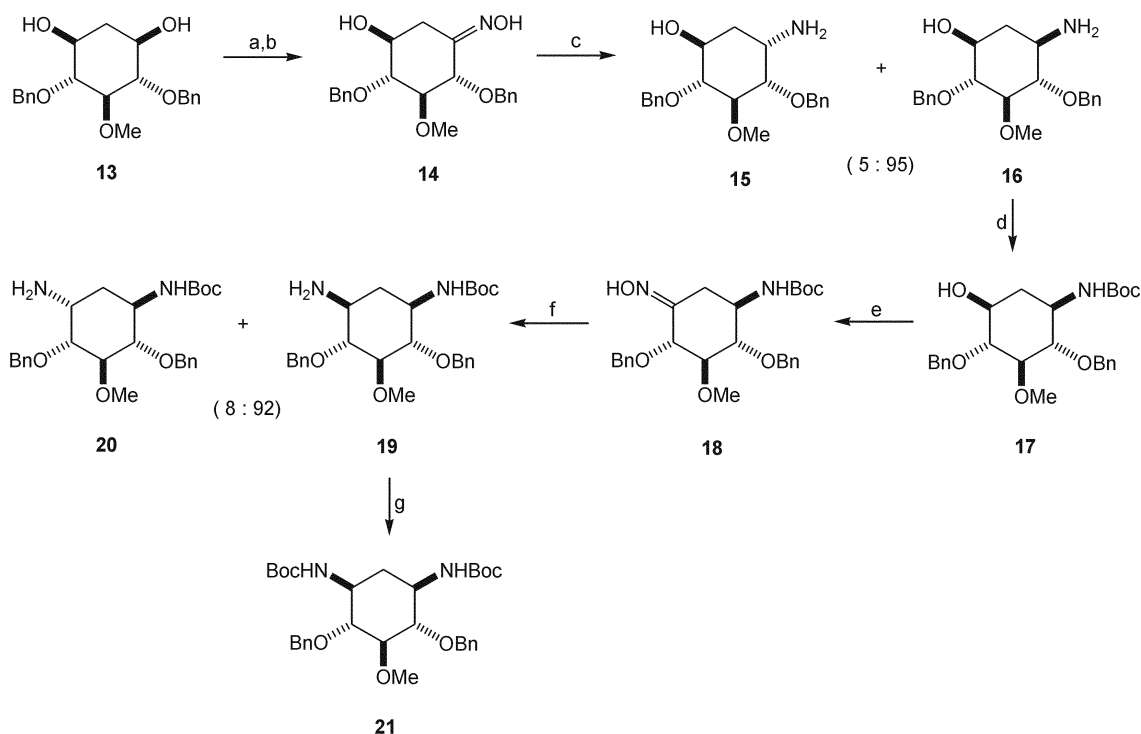
Scheme 2 7 . Reagents and Conditions: (a) PCC, \text{CH}_2\text{Cl}_2 , rt; (b) \text{H}_2\text{NOH}\cdot\text{HCl} , pyridine, two steps 85%; (c) \text{LiAlH}_4 , THF, reflux, 84%; (d) (\text{Boc})_2\text{O} , \text{Et}_3\text{N} , 100%; (e) same as (a) and (b), 80%; (f) same as (c), 80%; (g) same as (d), 100%.
