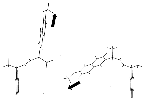
Figure 4. The conformations of the model compounds of (R,S)-CSP 1 (left) and (S,S)-CSP 1 (right). The conformations shown are consistent with those for (R)- or (S)-N-acyl- \alpha -naphthylethylamine and (S)-naproxen amide proposed previously. 10,3e The solid arrows indicate the direction of the connecting tether of the CSPs.
