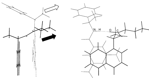
Figure 3. The proposed chiral recognition model viewed from the front side (left) and from the right side (right) for resolving N-(3,5-dinitrobenzoyl)- \alpha -phenylethylamine 2a on CSP 4 . The conformations of the model compound of CSP 4 , (R)-N-propanoyl- \alpha -naphthylethylamine (represented with thick lines), and (R)-N-(3,5-dinitrobenzoyl)- \alpha -phenylethylamine (represented with thin lines) shown in the drawing have been proposed in the previous studies. 8 The solid arrow indicates the direction of the connecting tether of the CSP. The empty arrow indicates the direction of the alkyl chain at the chiral center of the (R)-analyte.
