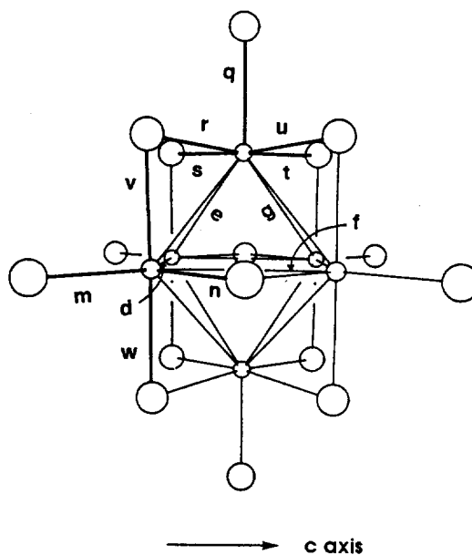
Figure 2. \text{Mo}_6\text{O}_{16} cluster unit having the same geometry as in the \text{KMo}_4\text{O}_6 solid. The labels m , n , and q-w indicate Mo-O distances, and d-g identify Mo-Mo distances.
