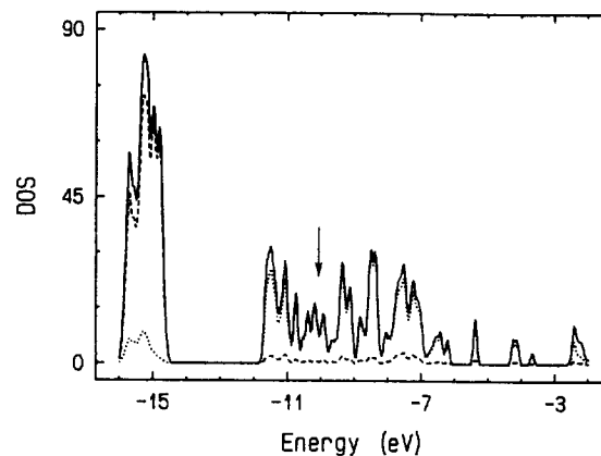
Figure 5. Plots of total DOS (solid line), Mo 4d contribution (dotted line) and O 2p contribution (dashed line) to the total DOS for the \text{Mo}_8\text{O}_{12}^{2-} slab of \text{KM}_2\text{O}_6 . The Fermi level is indicated by the arrow.
