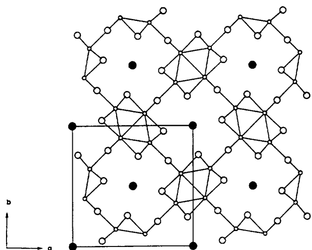
Figure 1. Projection of the tetragonal \text{KMo}_4\text{O}_6 structure viewed along the c axis. The small and large open circles represent Mo and O atoms, respectively. The \text{K}^+ ions are shown as darkened circles.
