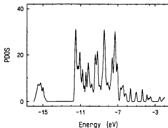
Figure 9. Plot of PDOS on 4 d orbitals for the double chain of Figure 7.
