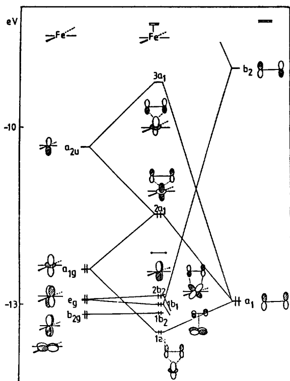
Figure 8. Correlation diagram of orbitals of \text{Fe}(\text{CO})_4(\text{C}_2\text{H}_4) with \text{D}_{4h} \text{Fe}(\text{CO})_4 and \text{C}_{2v} \text{H}_4 .
