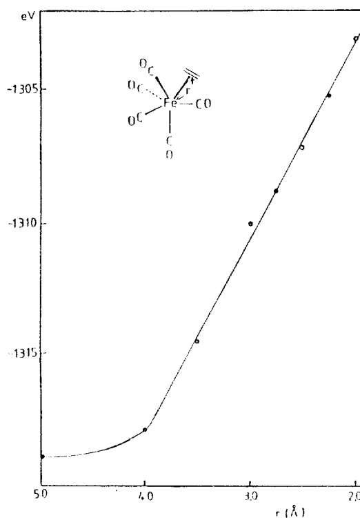
Figure 11. Potential curve for the distance between ethylene and iron [ \text{C}_1 \text{Fe}(\text{CO})_5 ].
