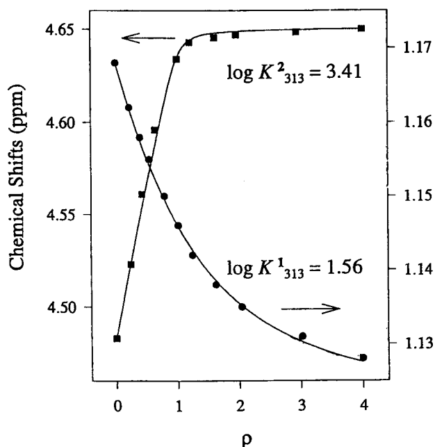
Figure 3. Plots of the chemical shifts for p - tert -butyl protons (filled circles) and \text{OCH}_2\text{CO} protons (filled squares) in ester 1 and 2, respectively, versus \rho in \text{THF-}d_8 at 313 K. The concentrations of 1 and 2 were maintained constant (0.04 M) while that of guest was varied.
