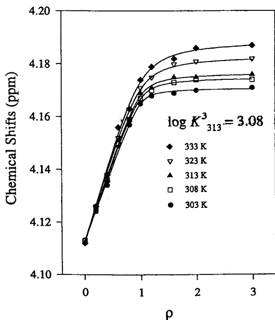
Figure 4. Plots of \text{OCH}_2\text{CO} proton chemical shifts in ester 3 versus \rho in \text{THF-}d_8 at several different temperatures. The concentration of 3 was maintained constant (0.04 M) while that of guest was varied.
