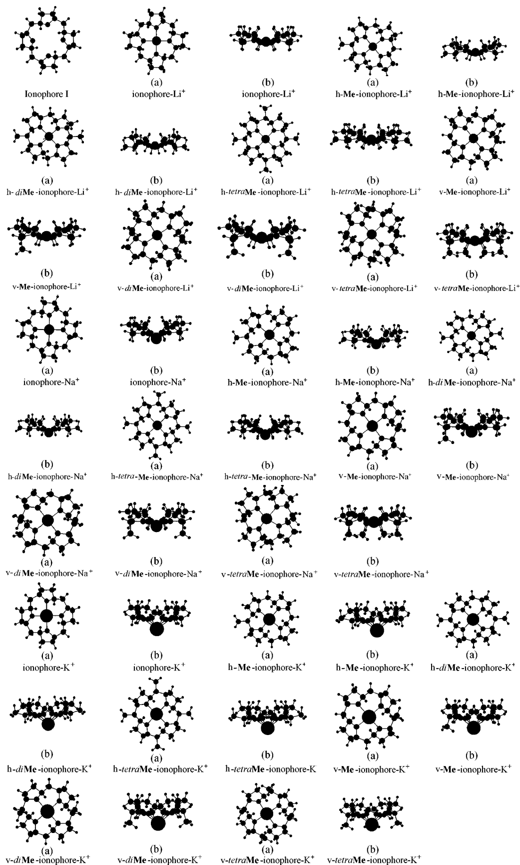
Figure 1. Geometric structures of 1,4,6,9,11,14,16,19-tetraoxacycloeicosane and ionophore-alkali metal cation complexes substituted by some methyl groups have been optimized using ab initio Hartree-Fock/6-31G* level. Top view is indicated as (a); Side view is indicated as (b).
