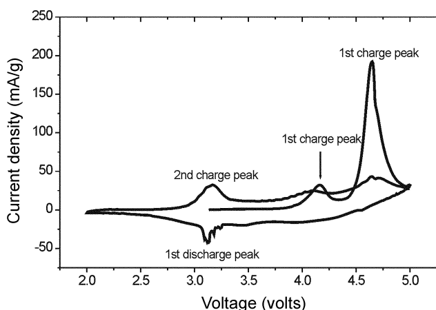
Figure 3. Cyclic voltammogram for \text{Li}[\text{Co}_{0.17}\text{Li}_{0.28}\text{Mn}_{0.55}]\text{O}_2 compound. The peaks detected during 1 st and 2 nd cycling are marked. Scan rate = 0.05 \text{ mV s}^{-1} .
