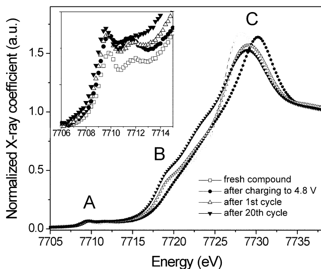
Figure 6. Co K-edge XANES spectra for \text{Li}[\text{Co}_{0.17}\text{Li}_{0.28}\text{Mn}_{0.55}]\text{O}_2 compound measured at different cyclic process.
