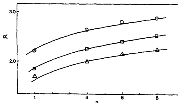
Figure 4. The chromatographic resolution of the (RR)/(SS) pairs of N-(3,5-dinitrobenzoyl)-amino acid-amino acid-O-(CH 2 ) n -H on CSP 1. Circle = Val-Val, Square = Leu-Val, Triangle = Phegly-Val. For chromatographic conditions, see text.
