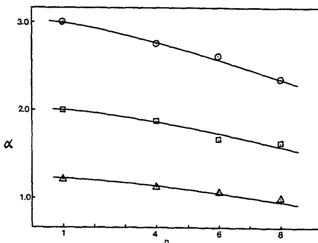
Figure 5. The chromatographic resolution of the (SS)/(RR) pairs of N-(3,5-dinitrobenzoyl)-amino acid-amino acid-O-(CH 2 ) n -H on CSP 2. Circle = Val-Val, Square = Leu-Val, Triangle = Phegly-Val. For Chromatographic conditions, see text.
