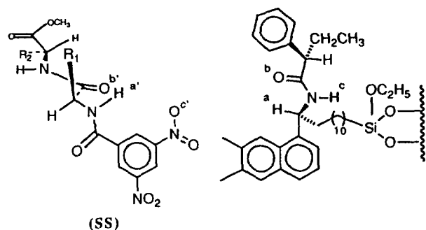
Figure 3. Overlapping the (SS)-enantiomer on CSP 3 with the \pi - \pi interaction between the 3,5-dinitrobenzoyl and the 6,7-dimethylnaphthyl group and the hydrogen-bondings (a'-b, b'-a and c'-c') shows the hydrogen-bonding process. In this process, the ester alkyl group of the (SS)-enantiomer is intercalating between the strands of bonded phase.
